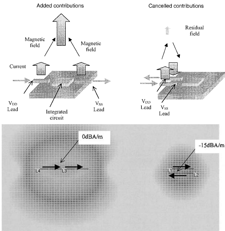
Figure 7-15. Using VDD/VSS pairs instead of placing VDD and VSS at each corner of the IC may lead to 15dB emission reduction
