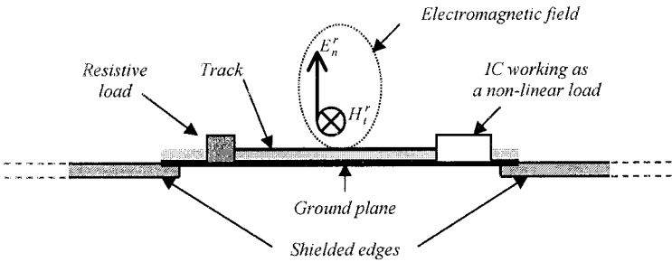
Figure 4-71. Test board illuminated by an electromagnetic wave.
