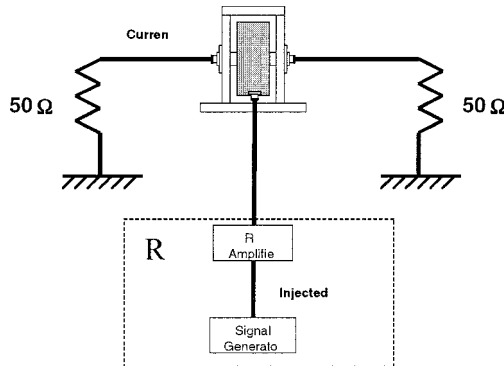
Figure 4-37. Schematized diagram of the calibration setup for the RF injection probe.
