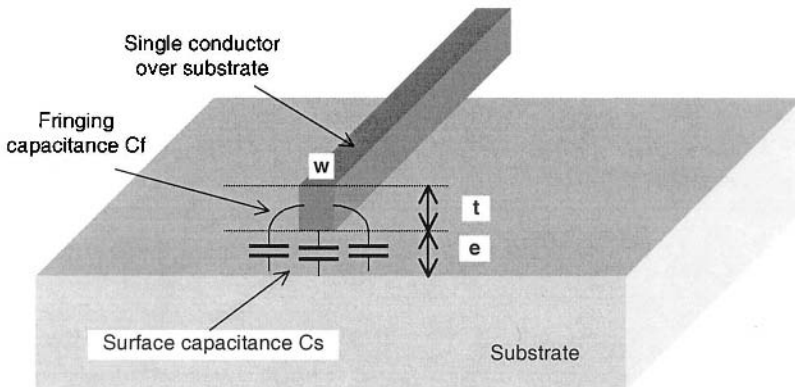
Figure 3-32. One conductor above a ground plane.
