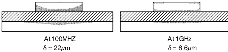
Figure 3-24. Current distribution in the 100 MHz to 1 GHz band.
