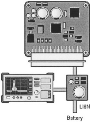
Figure 6-80. Measurement system.
