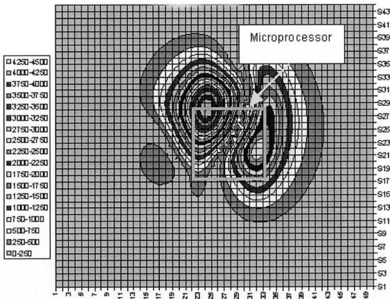
Figure 5-121. Simulated magnetic field.
