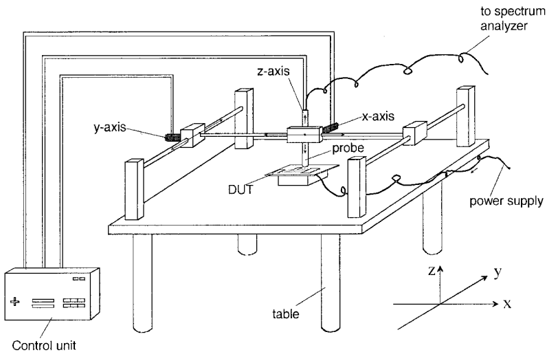
Figure 4-14. Example of a near-field scanner setup.
