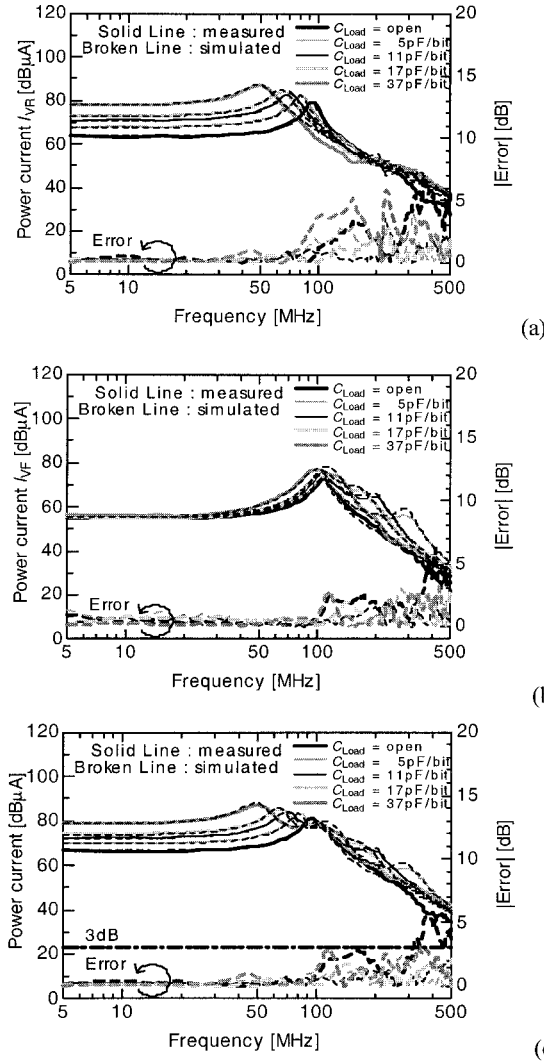
Figure 5-80. Noise current spectra and its simulations with LECCS-I/O model (a) Rising, (b) Falling, and (c) Total current spectra.
