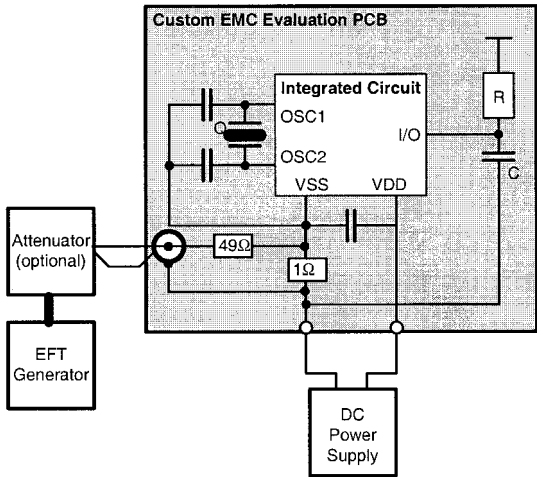
Figure 4-62. Reference injection test setup.
