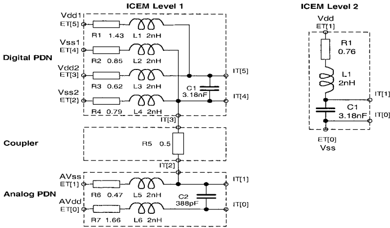
Figure 5-36. PDN component description levels.
