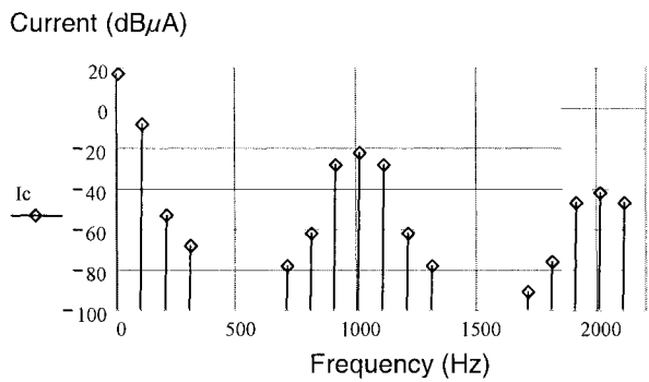
Figure 6-75. Simulation results for the collector current I_c of an analog multiplier with a 100 Hz input signal and affected by a 1 kHz bias current disturbance.
