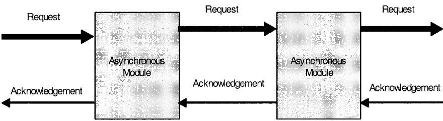
Figure 7-4. Handshake- based communication between modules.
