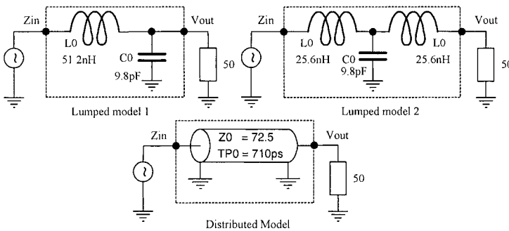
Figure 3-20. Models used for time- and frequency-domain analyses.
