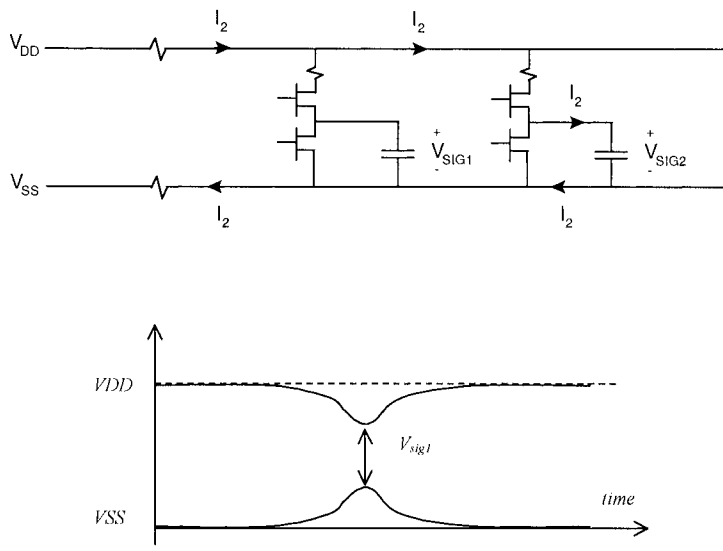
Figure 1-4. Two totem-pole CMOS drivers sharing a power bus.
