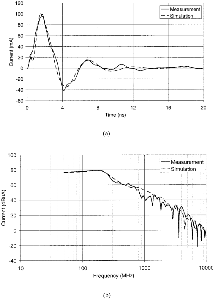
Figure 6-8. Comparison between on-chip measurement and simulation of the current through RVDD for the NORM core: (a) Time-domain results, (b) Frequency-domain results, calculated by FFT.
