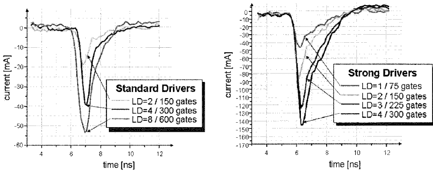
Figure 6-26. Measured switching current in EMU: standard (left) and strong drivers (right).
