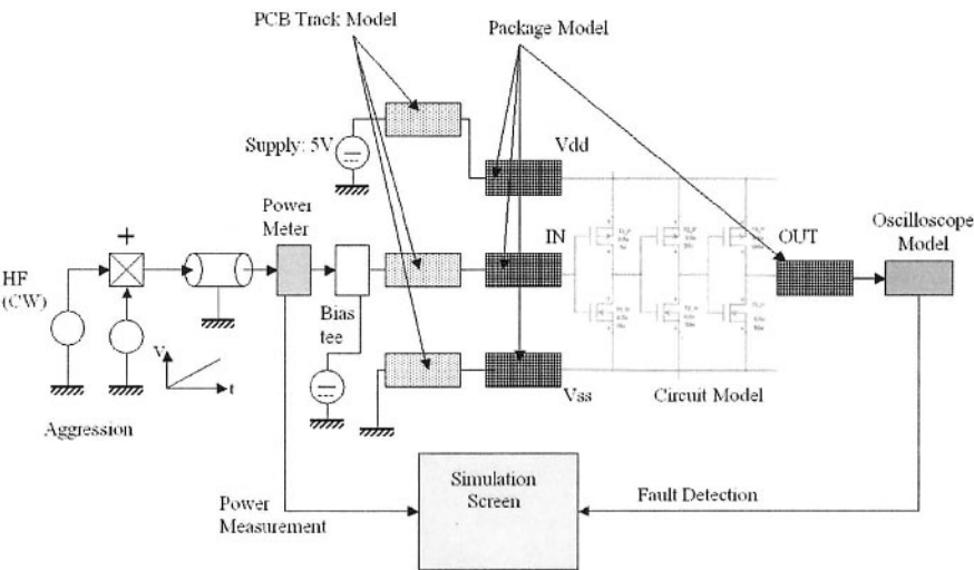
Figure 6-54. Synoptic of aggression bench model.
