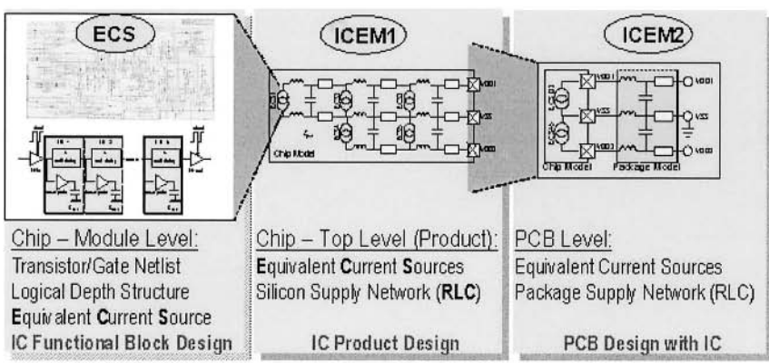
Figure 6-15. Emission model types.
