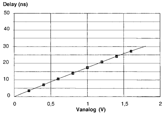
Figure 4-80. Delay cell characterization vs. Vanalog voltage control.
