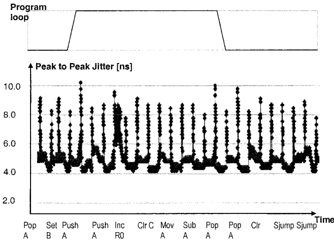
Figure 4-66. TDMA response from a microcontroller as function of the codes running.
