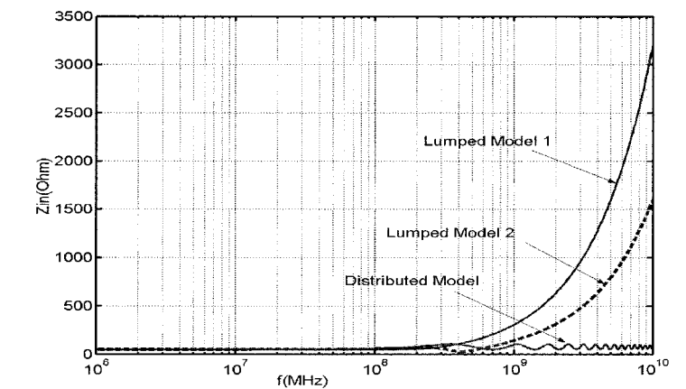
Figure 3-21. Impedance of the three models.
