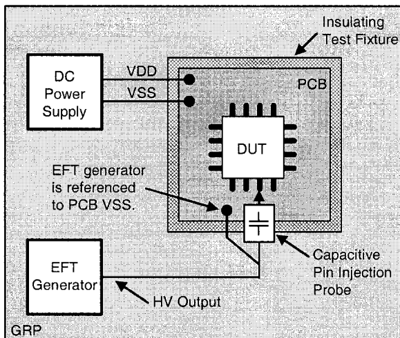
Figure 4-58. Pin injection test setup (top view).
