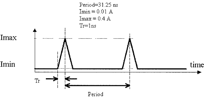
Figure 5-53. ICEM Current generator.
