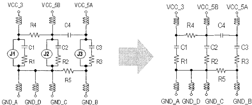
Figure 6-87. LECCS Model for EMI (left) and EMS (right)
