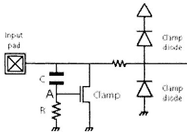
Figure 5-84. I/O protection by coupled-gate NMOS transistor.
