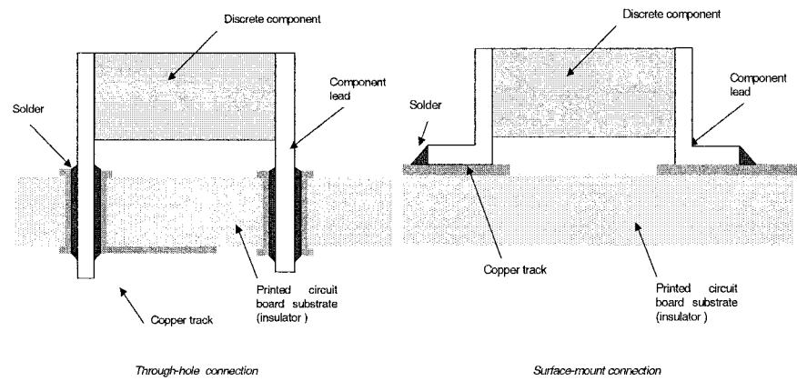
Figure 5-17. PCB technologies.
