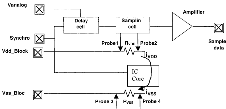
Figure 4-78. Principles of the on-chip sampling of core current.
