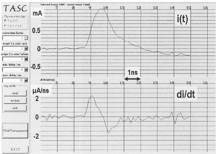
Figure 6-23. Current measurement on TASC
