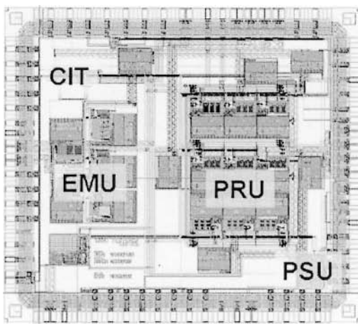
Figure 6-16. TASC modules.
