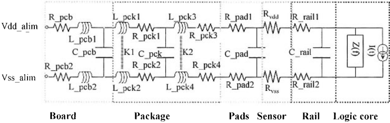
Figure 6-2. Complete model of the CESAME test chip.
