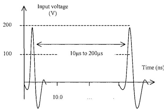
Figure 4-54. Electrical Fast Transient.
