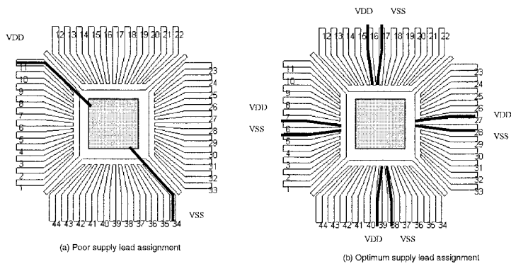
Figure 7-14. Improved VDD/VSS assignment
