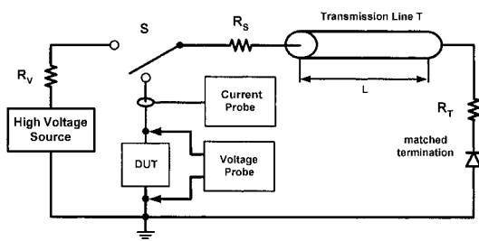
Figure 5-10. Schematic of a TLP test system ( R_V=1\text{ M}\Omega , R_S=50\text{ }\Omega - 1000\text{ }\Omega , R_T=50\text{ }\Omega ).
