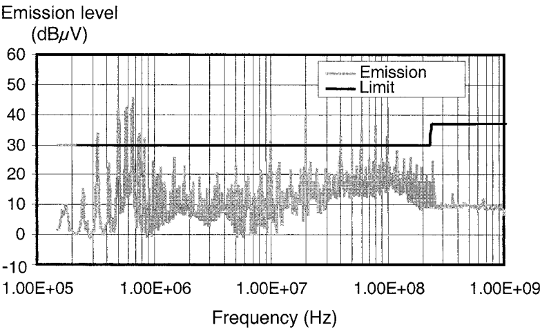
Figure 4-33. Conducted measurement using WBFC.
