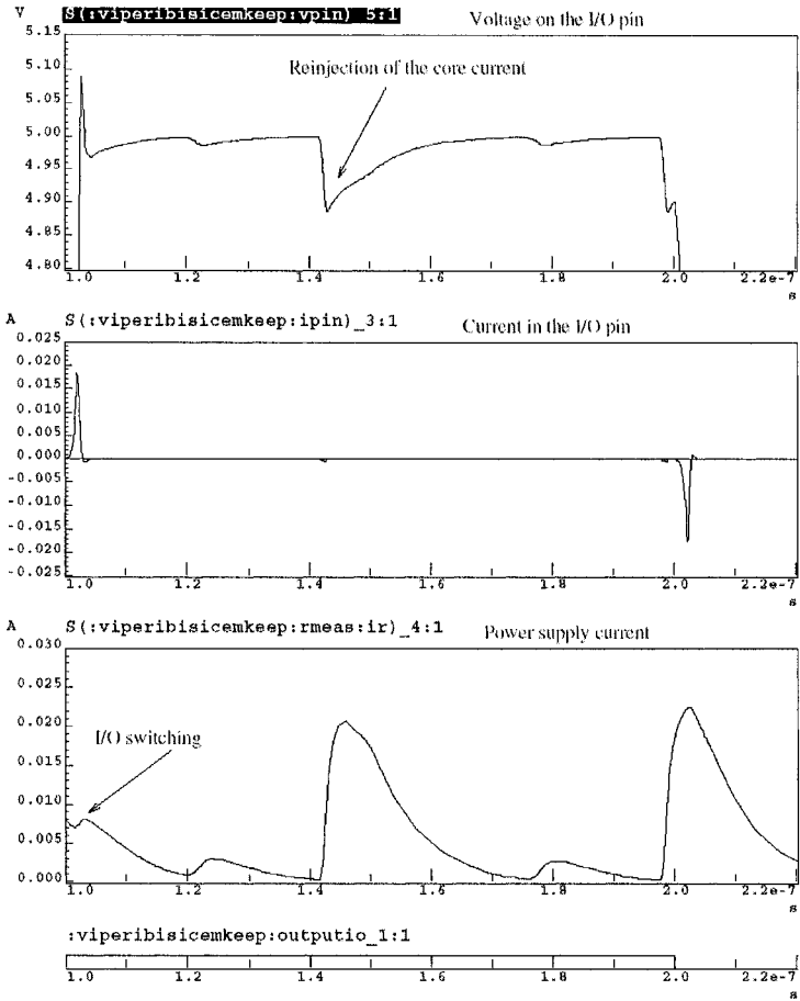
Figure 6-41. Core-I/O coupling.
