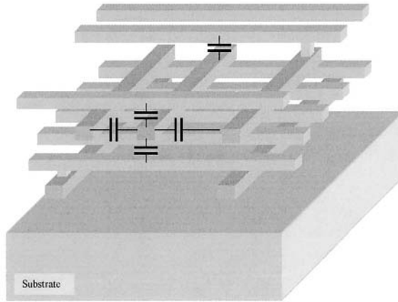
Figure 3-30. One interconnect is coupled to other conductors in several ways, both lateral and vertical.
