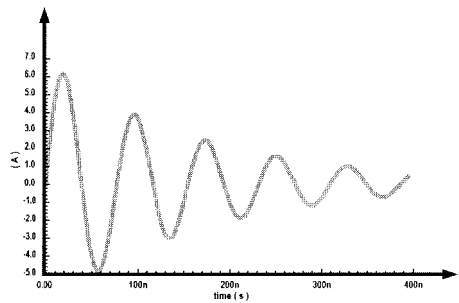
Figure 5-7. Current waveform of a 400V MM ESD discharge as specified in AEC-Q100-003-REV-F.
