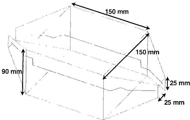
Figure 4-4. Typical dimensions of a 1-GHz TEM cell.
