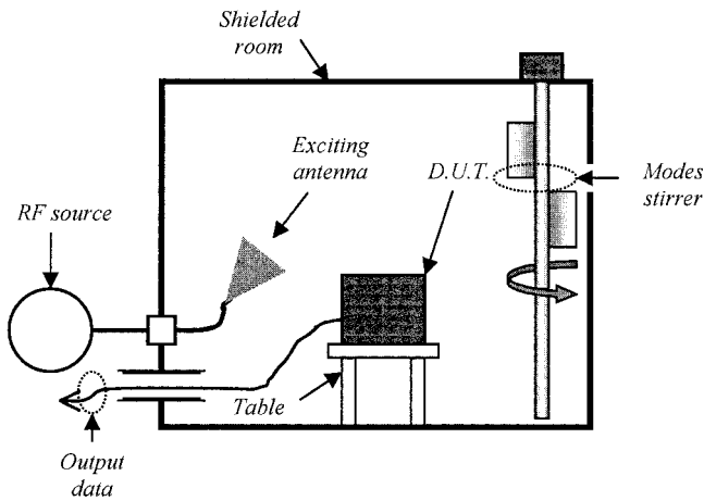
Figure 4-75. Mode-stirred reverberating chamber.
