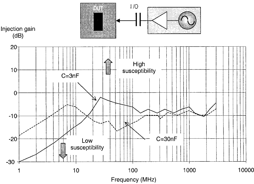
Figure 7-23. Effect of on-chip capacitance on transfer gain from the RFI source and the IC core.
