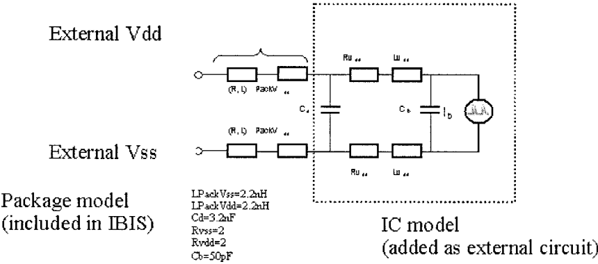
Figure 5-52. 68HC12 D60 ICEM model.
