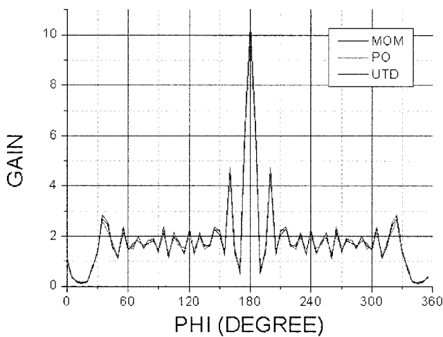
Figure B-11. Comparison of MoM, PO and UTD results on a rectangular reflector case.
