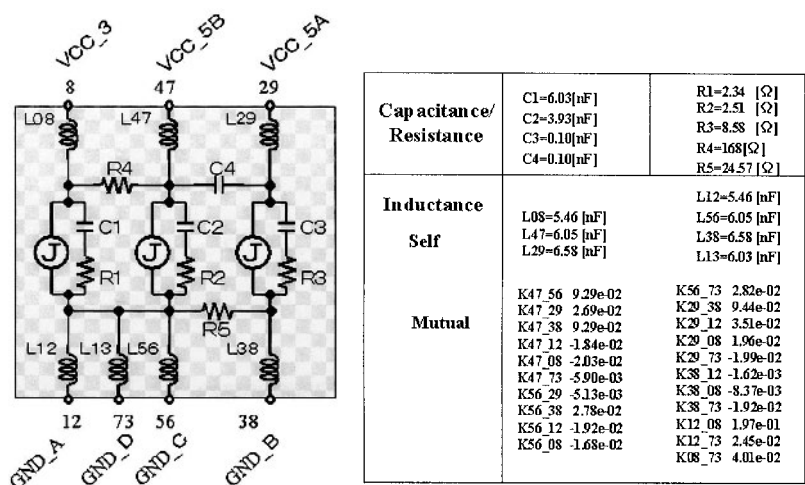
Figure 6-77. LECCS model of a microcontroller
