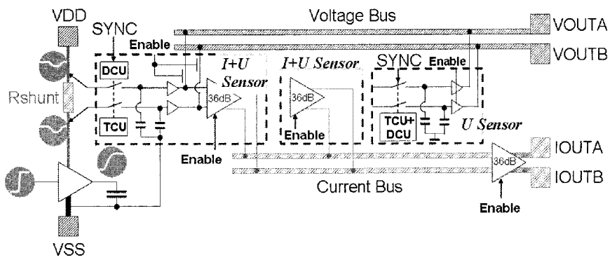
Figure 6-20. Voltage and current sensing and amplifying circuit.
