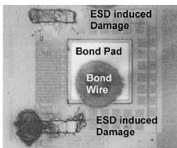
Figure 5-1. Detailed view of melted metal traces due to ESD stress.
