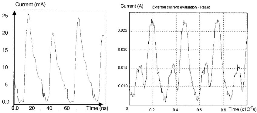
Figure 6-37. simulated (left) and measured (right) external currents of the CPU core
