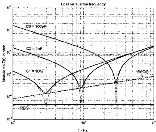
Figure 3-27. Losses versus frequency.
