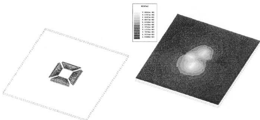
Figure B-25. Prediction of the near-field radiation from an integrated circuit.
