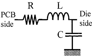
Figure 6-44. Package model from IBIS file.
