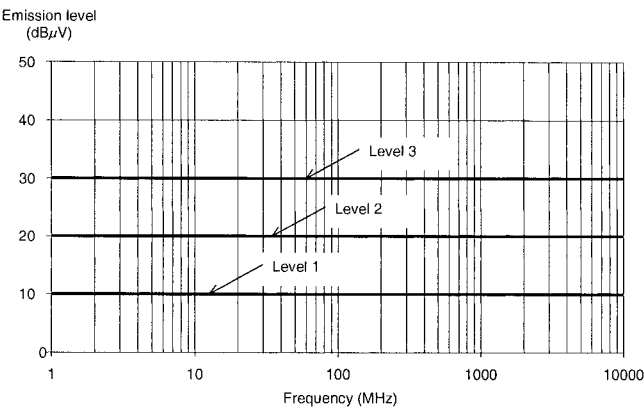
Figure 4-85. Maximum emission levels specified in TEM cell.
