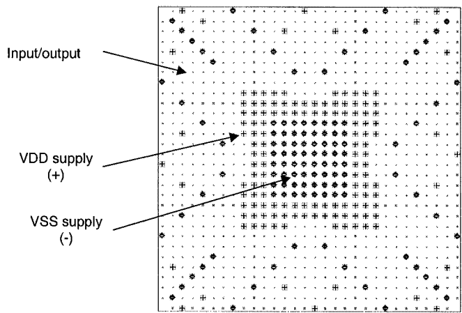
Figure 7-17. VDD/VSS assignment for a VIRTEX programmable device.
