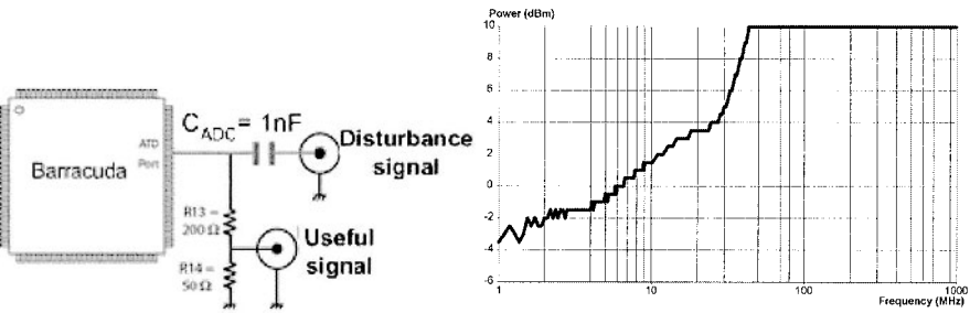
Figure 6-68. Immunity measurement results.
