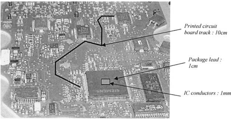
Figure 4-25. Test board example and associated conductor dimensions.
