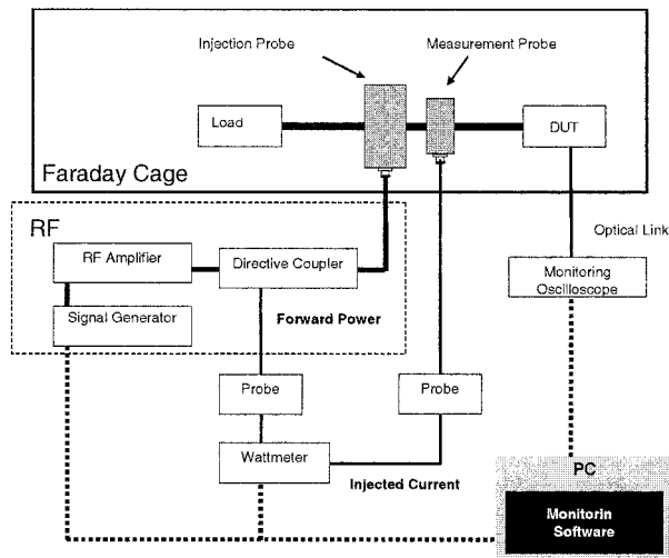
Figure 4-40. BCI measurement test setup.
