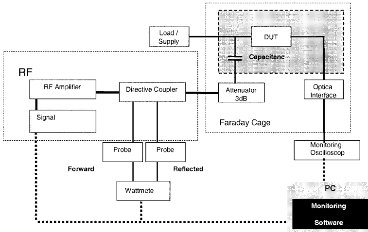
Figure 4-49. DPI measurement setup with attenuator.
