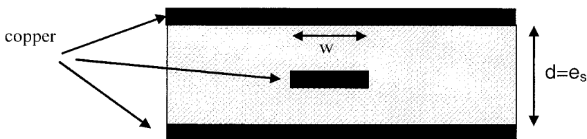
Figure 5-21. Stripline configuration.
