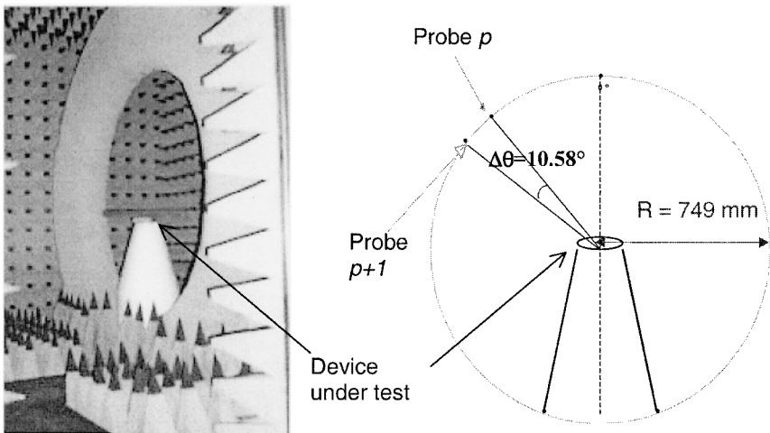
Figure 4-16. Photograph of the spherical test setup at IETR Rennes, France.
