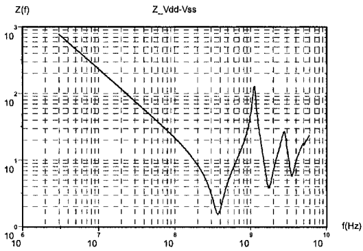
Figure 6-50. Simulation of impedance seen between V_{dd} and V_{ss} pins.
