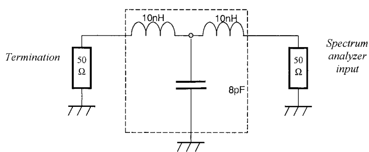
Figure 5-114. Simple TEM cell model.
