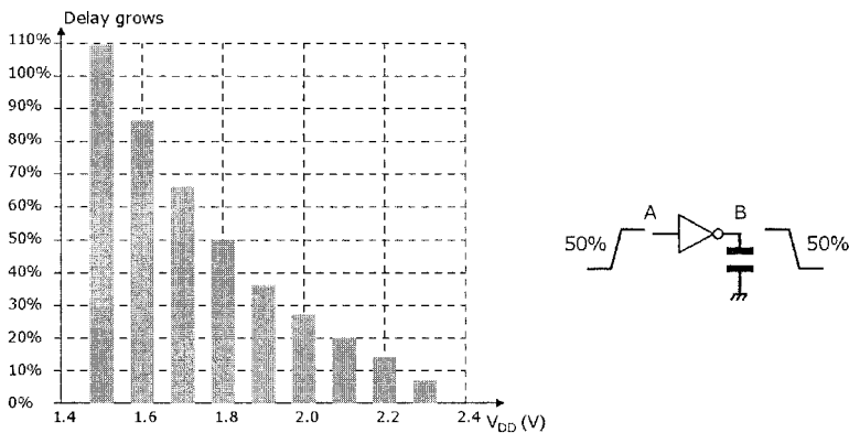
Figure 5-92. The distribution delay is significantly increased with the decrease of the power supply voltage.
